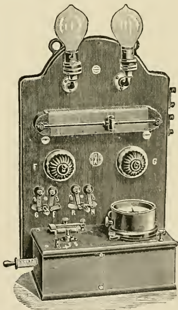
FIG. 116. — Switch board for shunt regulation.
